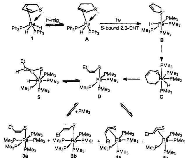
Scheme IV. Proposed Mechanism for the Formation of 3 and 4
