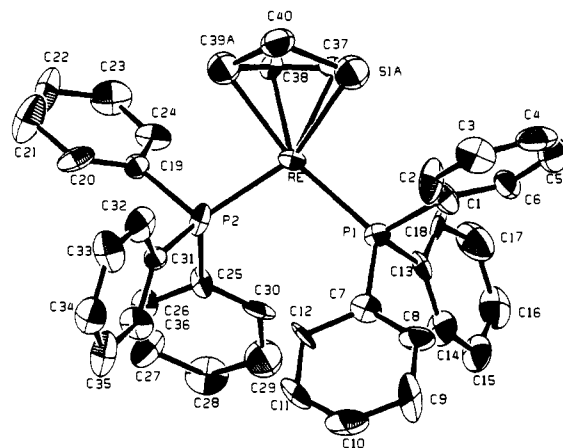
Figure 3. ORTEP diagram of 1 with the thermal ellipsoids shown at 50% probability. The hydride ligands were not located.
