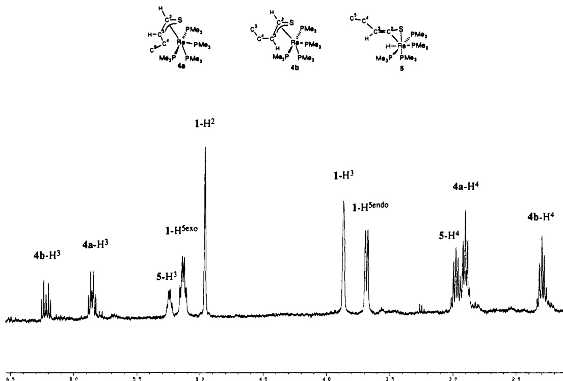
Figure 6. ^1H NMR spectrum of the same sample as in Figure 5 after removal of solvent and excess PMe_3 , showing the disappearance of 3 and the appearance of 5 .
